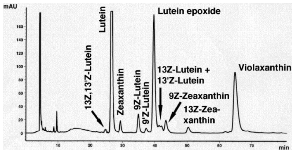
Figure 2. Carotenoid HPLC profile of an extract from green beans on a silica-based nitrile-bonded column employing eluent A. Conditions are described in the text.
